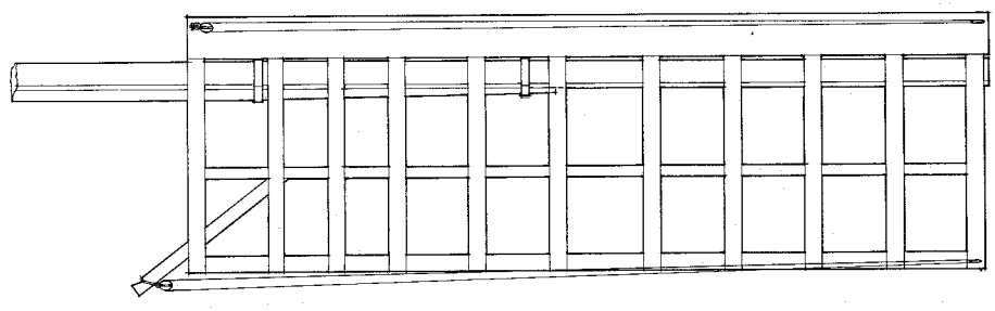
OUTSIDE ELEVATION OF WIND VANE
